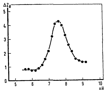
FIGURE 4: Difference in protons bound by bovine serum albumin in the presence and absence of calcium ions. The curve was obtained from the data of Figure 2.
