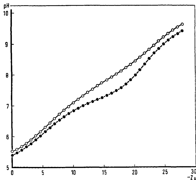
FIGURE 2: Normal titration curves of bovine serum albumin in KCl (O) or \text{CaCl}_2 (●). Ionic strength 0.06; protein concentration 2%; temperature 24.9^\circ .
