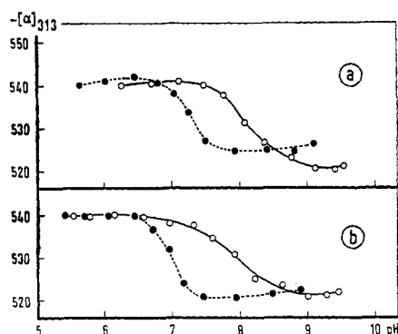
FIGURE 1: Specific rotation at 313 nm as a function of pH in the presence of KCl (○) or \text{CaCl}_2 (●). Ionic strength 0.06 (a) or 0.20 (b). Protein concentration 0.5%; temperature 25°.
