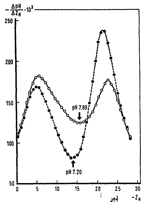
FIGURE 3: Differential titration curves of bovine serum albumin in KCl (O) or \text{CaCl}_2 (●). Ionic strength 0.06; protein concentration 2%; temperature 24.9^\circ .
